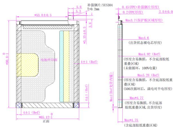
Battery (Unit: mm)
