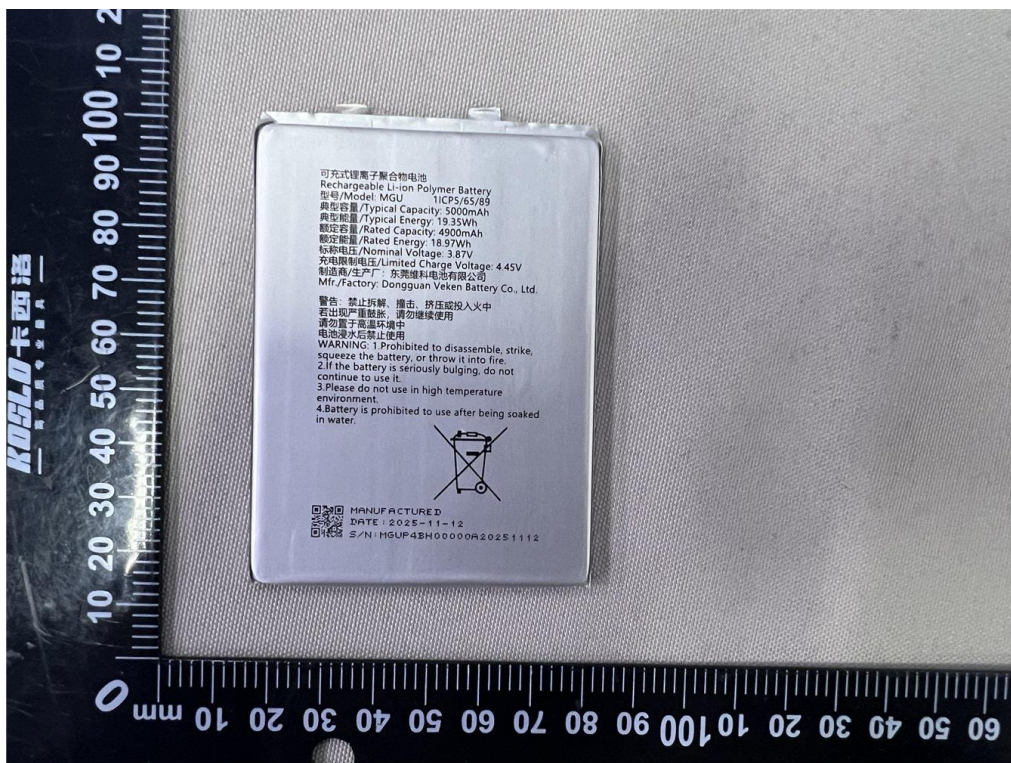
Figure 8 Back view of cell
